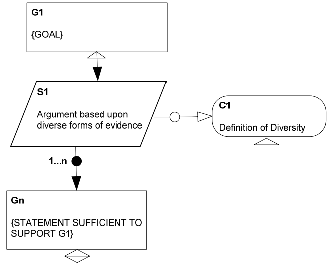
Figure 7. Diverse Argument Safety Case Pattern [8]
