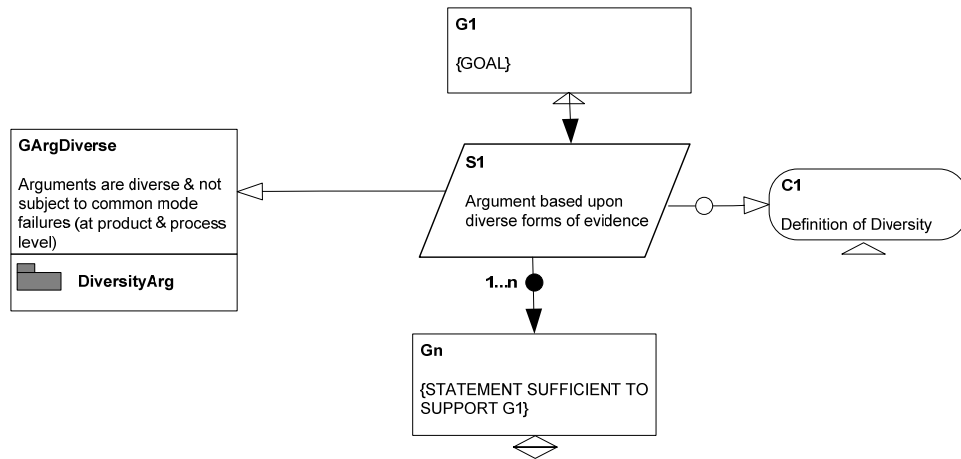
Figure 8. Extended Diverse Argument Safety Case Pattern
