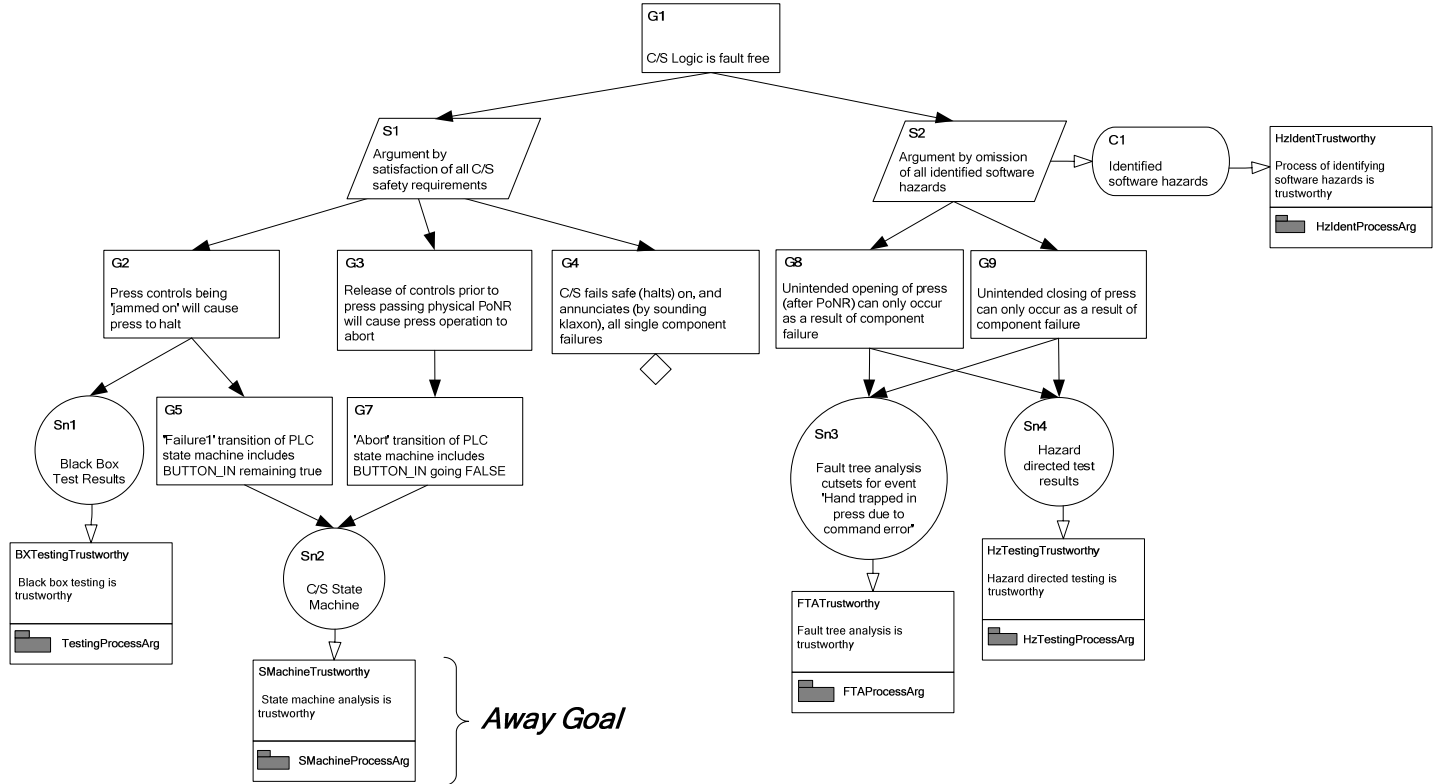
Figure 4. Process Argument Extension
