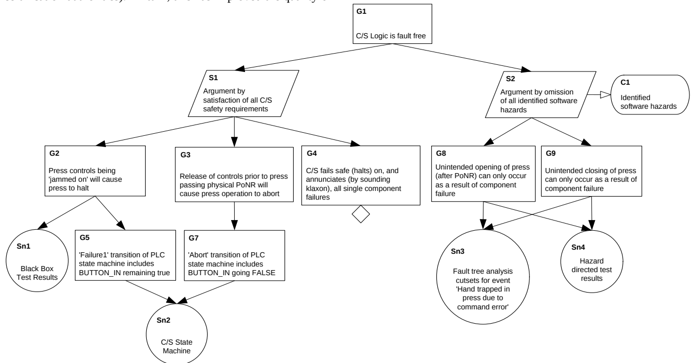
Figure 3. An Example Goal Structure
