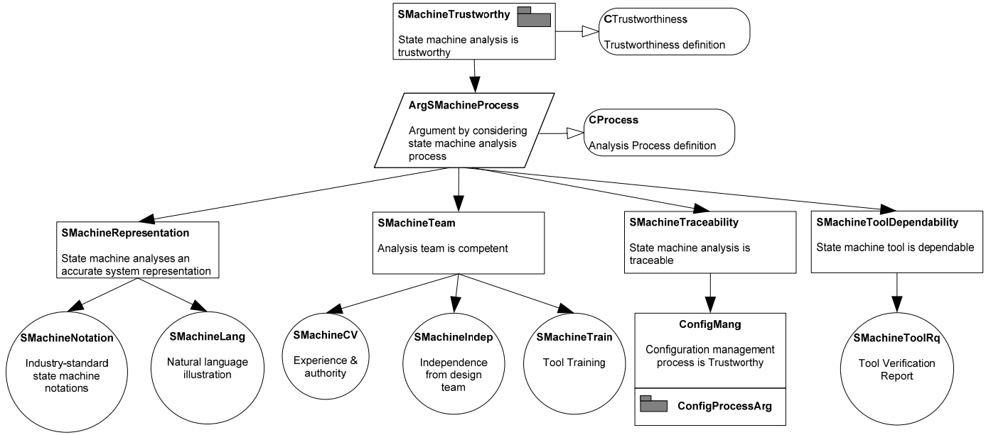
Figure 6. State Machine Process Argument
