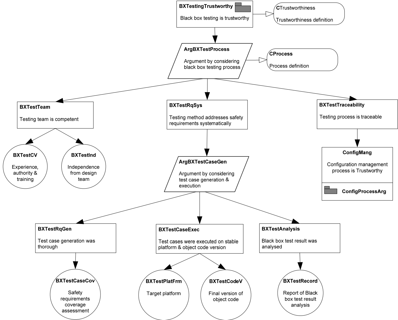
Figure 5. Black-Box Process Argument
