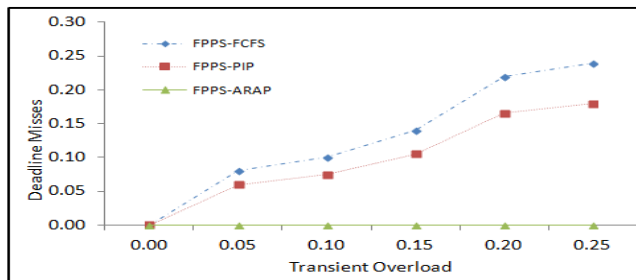
Figure 8: Hard Real-Time task miss rate (vxWorks)
